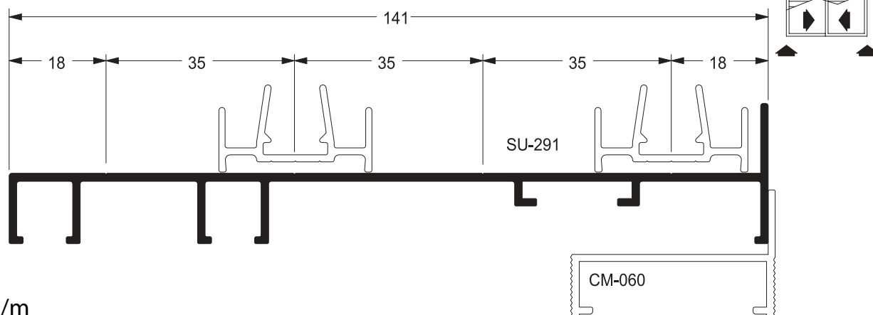
Marco lateral / correr 4
